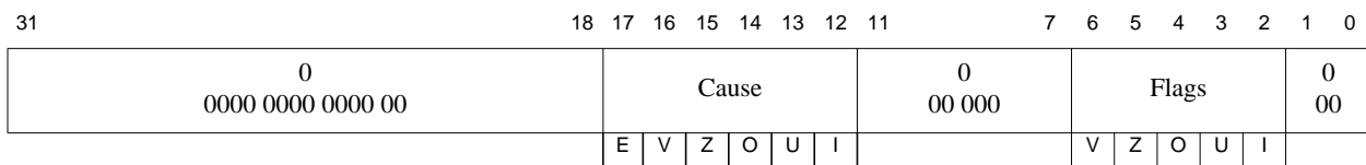
Figure 5-16 FEXR Register Format
