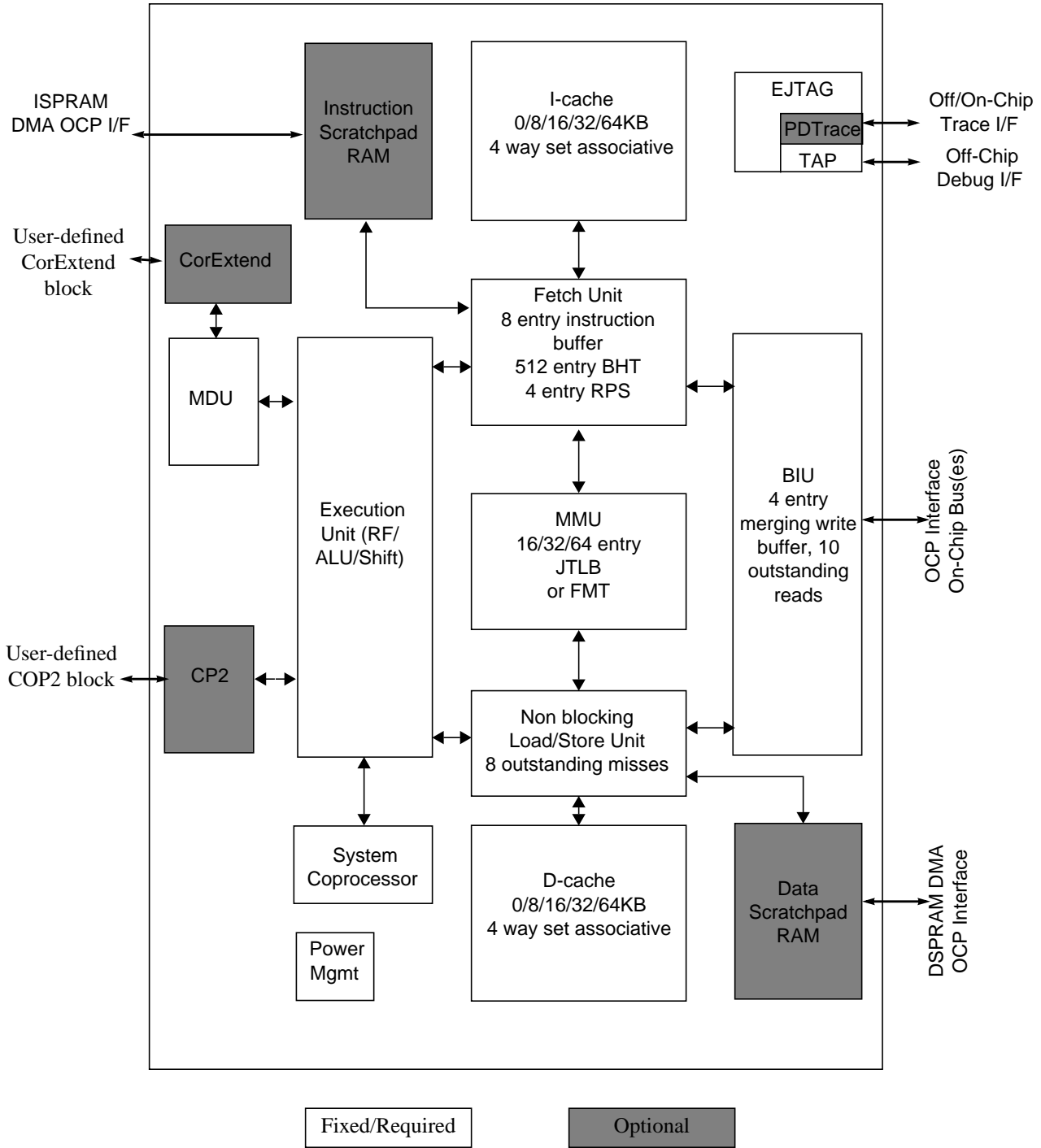
Figure 1 24KEc™ Core Block Diagram
