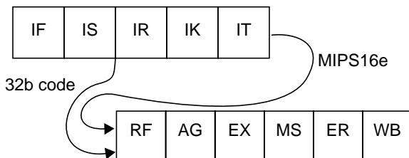
Figure 2 24KEc™ Core Pipeline
